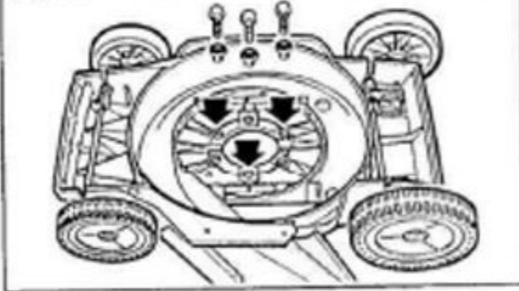
MOTOR MOUNT (Bottom View): Items 35, 36 assembled in 3 locations indicated.
